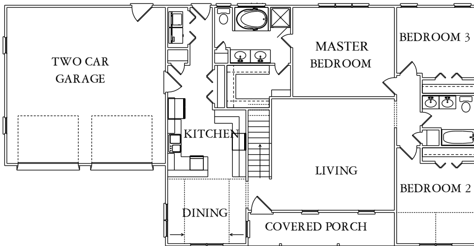
1ST FLOOR
